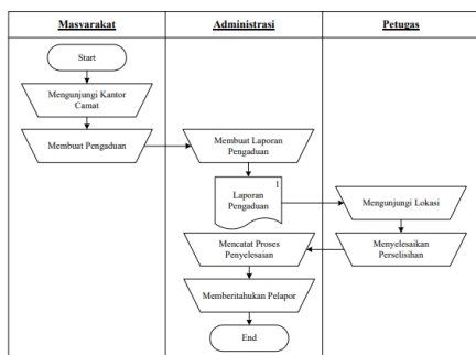
Gambar 3 Flowmap Sistem Berjalan
