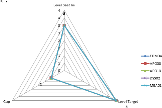
Gambar 8. Capability Level
