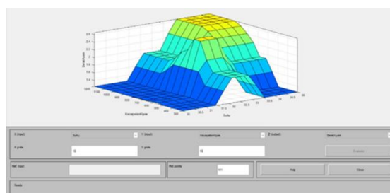
Gambar. 7 Surface Viewer
