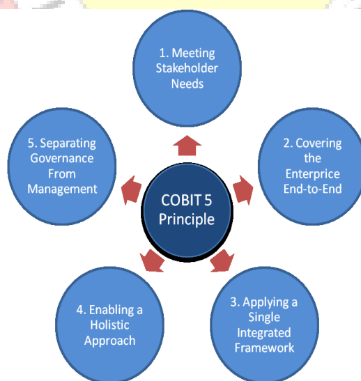
Gambar 1. Prinsip Cobit 5
