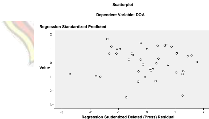
Gambar 4 Scatterplot
