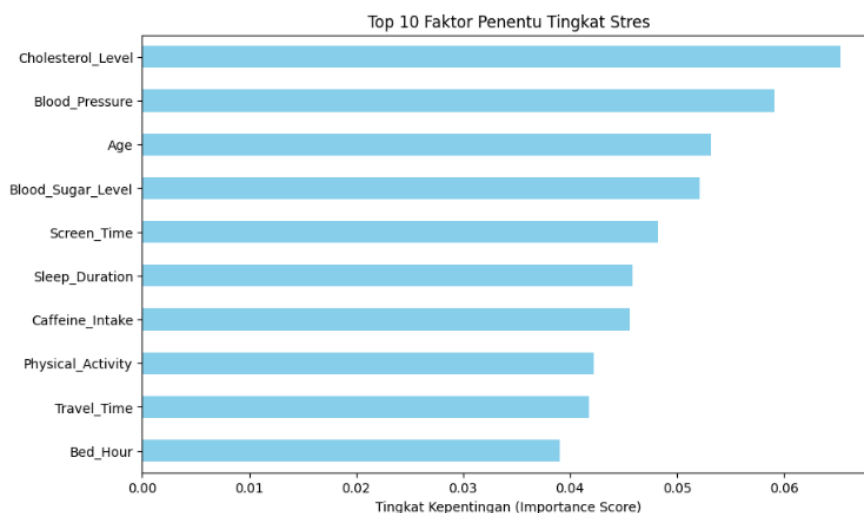
Gambar 5. Hasil Feature Importance
