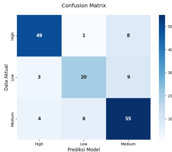
Gambar 4. Hasil Confusion Matrix
