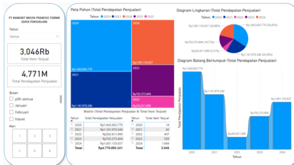
Gambar 10 Dashboard
