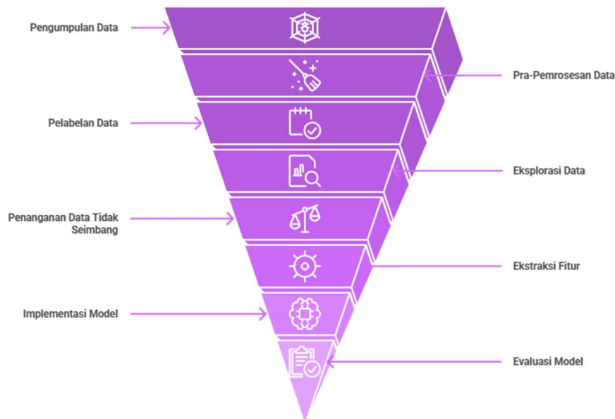
Gambar 1. Flowchart Penelitian
