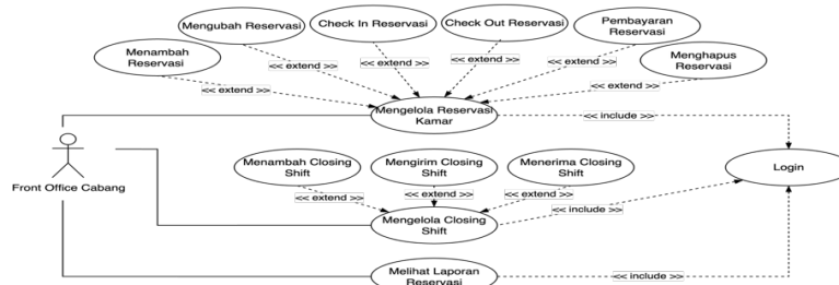
Gambar 4. Use Case Diagram Aktor Front Office Cabang
