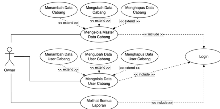
Gambar 2. Use Case Diagram Aktor Owner
