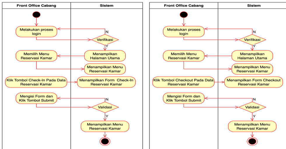
Gambar 8. Activity Diagram Check In dan Chekout Reservasi Kamar (Dari Kiri)
