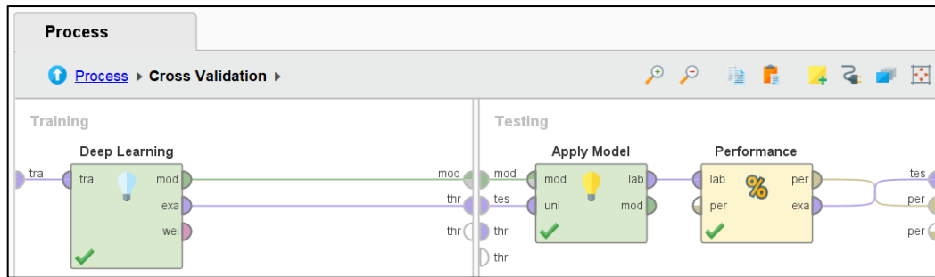
Gambar 8 Deep Learning
