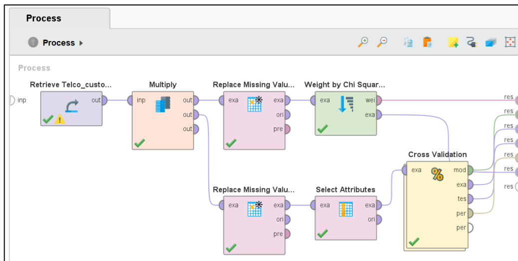
Gambar 6 Chi Square
