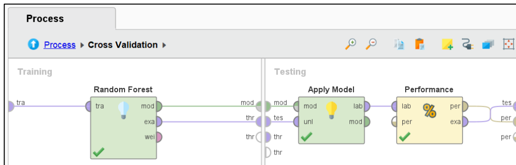
Gambar 9 Random Forest
