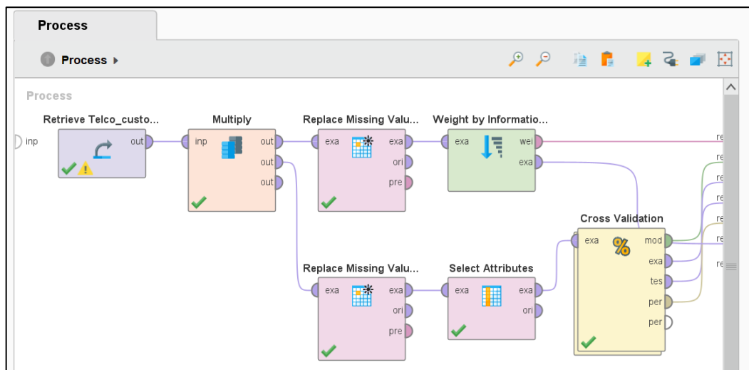
Gambar 7 Information Gain
