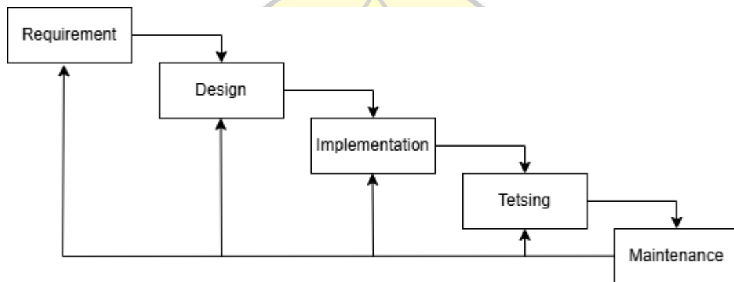
Gambar 1 Metode Waterfal
