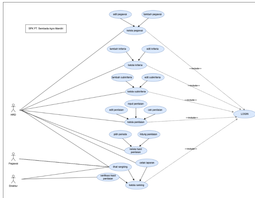
Gambar 1. Usecase Diagram
