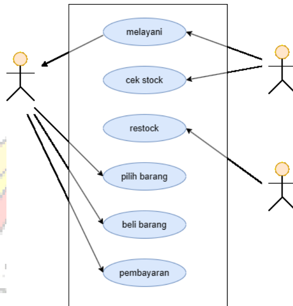
Gambar 2. Diagram Use Case Pembelian Offline
