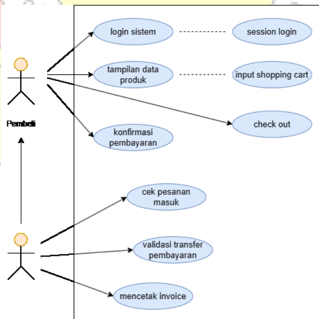
Gambar 3. Diagram Use Case Pembelian Online
