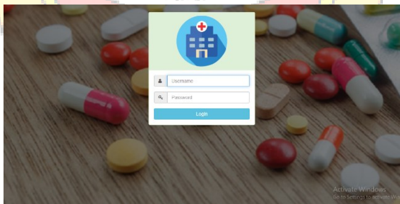
Gambar 4. Form Login
