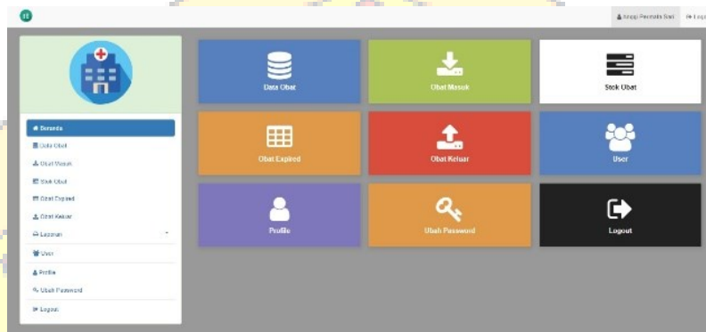
Gambar 5. Halaman Dashboard
