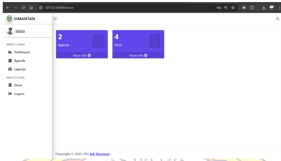
Gambar 7. Halaman Dashboard
