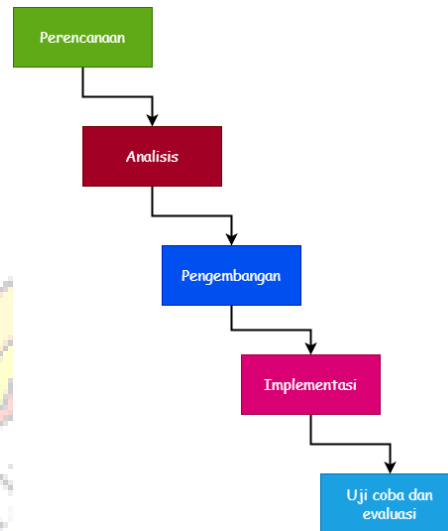
Gambar 1. Metode Waterfall
