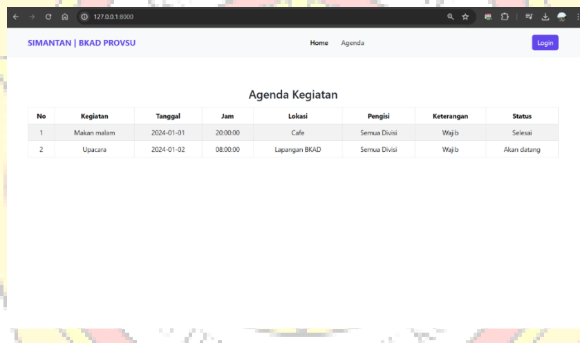
Gambar 11. Halaman Website
