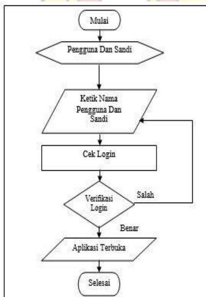
Gambar 4 Flowchart Form Login
