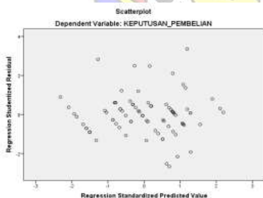
Gambar 1.3 Gambar Scatter Plot
