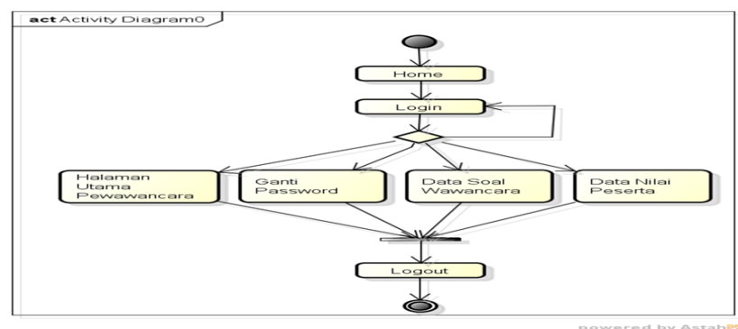
Gambar 4 Activity Diagram Pewawancara
