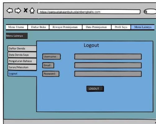
Gambar 13.1 Halaman logout
